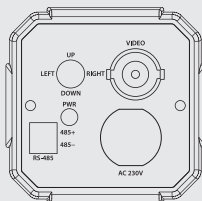
AC230V
