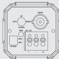
DC12V
